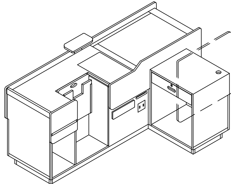
I1 01 ISOMETRIC VIEW: SB-208 CHECKOUT L/H SHOWN SCALE: NOT TO SCALE
