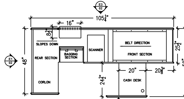
P1 01 PLAN VIEW: SB-230 LEFTHAND CHECK STAND SCALE: 3/8" = 1'-0"
