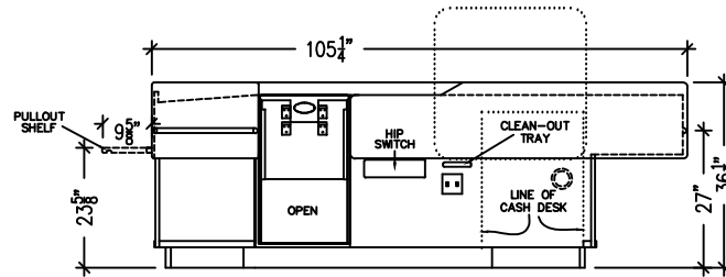
E2 01 INSIDE ELEVATION: SB-230 LEFTHAND CHECK STAND SCALE: 3/8" = 1'-0"
