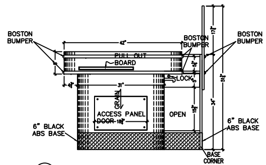
E4 01 REAR ELEVATION: SB-40-PED CHECKOUT SCALE: 1" = 1'-0"
