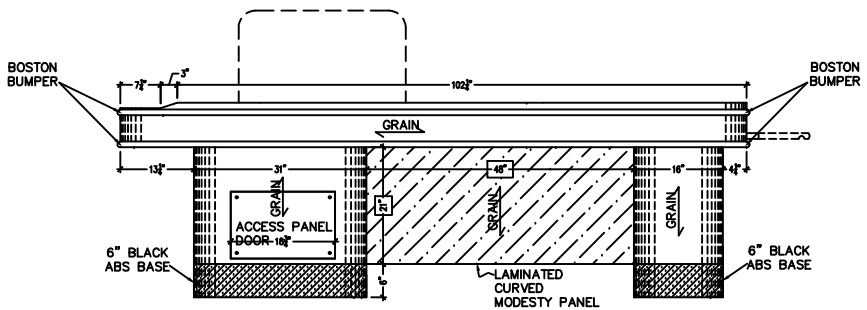
E3 01 ELEVATION: SB-40-PED CHECKOUT CUSTOMER SIDE SCALE: 1" = 1'-0"
