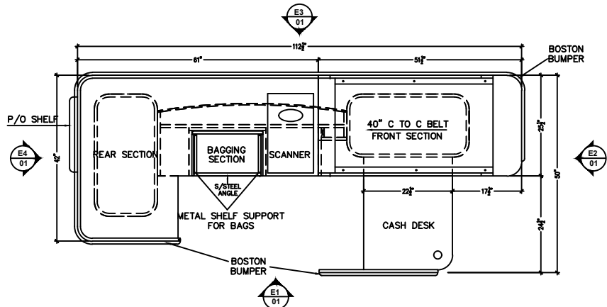
P1 01 PLAN VIEW: SB-40-PED CHECKSTAND L/H SHOWN SCALE: 1" = 1'-0"
