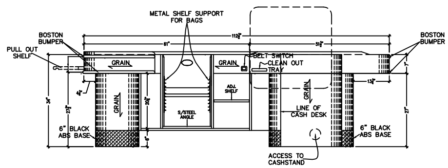
E1 01 ELEVATION: SB-40-PED CHECKOUT CASHIER SIDE SCALE: 1" = 1'-0"
