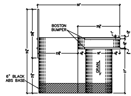
E2 01 REAR ELEVATION: SB-40-PED CHECKOUT SCALE: 1" = 1'-0"
