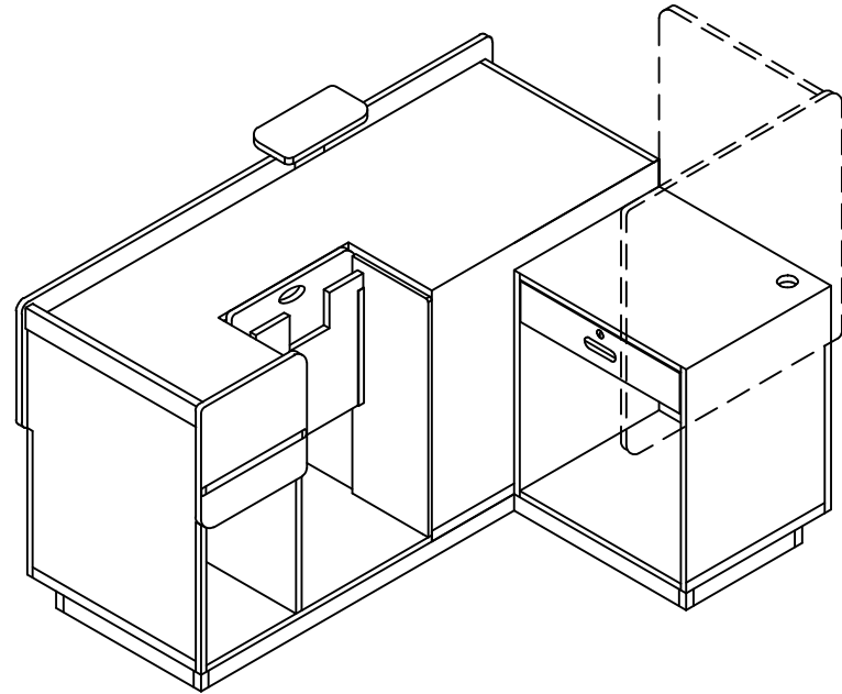
I1 01 ISOMETRIC VIEW: SB-142 CHECKOUT L/H SHOWN SCALE: NOT TO SCALE
