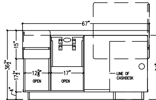
E2 01 INSIDE ELEVATION: SB-142 CHECKOUT L/H SHOWN SCALE: 3/8" = 1'-0"
