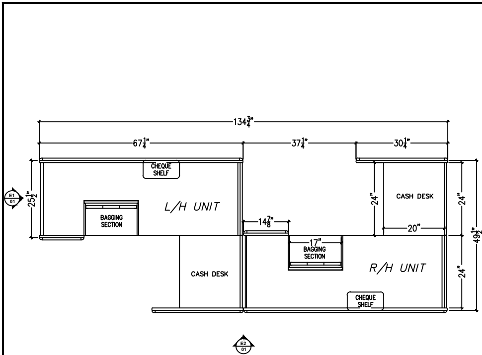
P1 01 PLAN VIEW: SB-142 CHECKOUT L/H AND R/H SHOWN SCALE: 3/8" = 1'-0"
