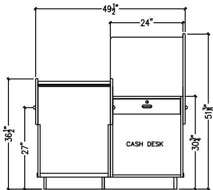
E1 01 END ELEVATION: SB-142 CHECKOUT L/H SHOWN SCALE: 3/8" = 1'-0"
