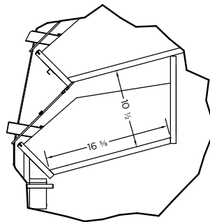
DETAIL D SCALE 1 / 8
