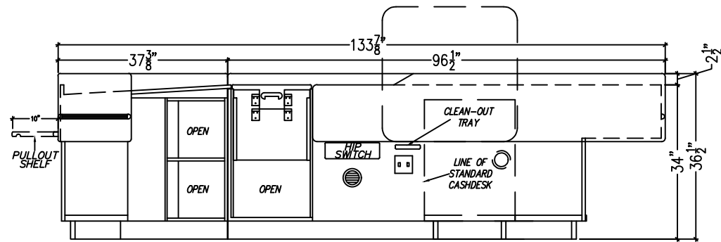
E2 01 INSIDE ELEVATION: SB-215 CHECKOUT L/H SHOWN SCALE: 3/8" = 1'-0"
