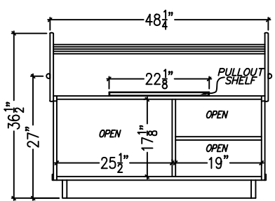
E1 01 END ELEVATION: SB-215 CHECKOUT L/H SHOWN SCALE: 3/8" = 1'-0"
