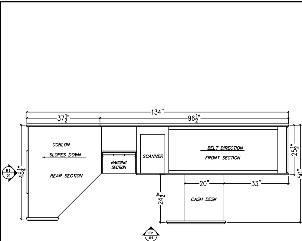
P1 01 PLAN VIEW: SB-215 CHECKOUT LEFT HAND SHOWN SCALE: 3/8" = 1'-0"
